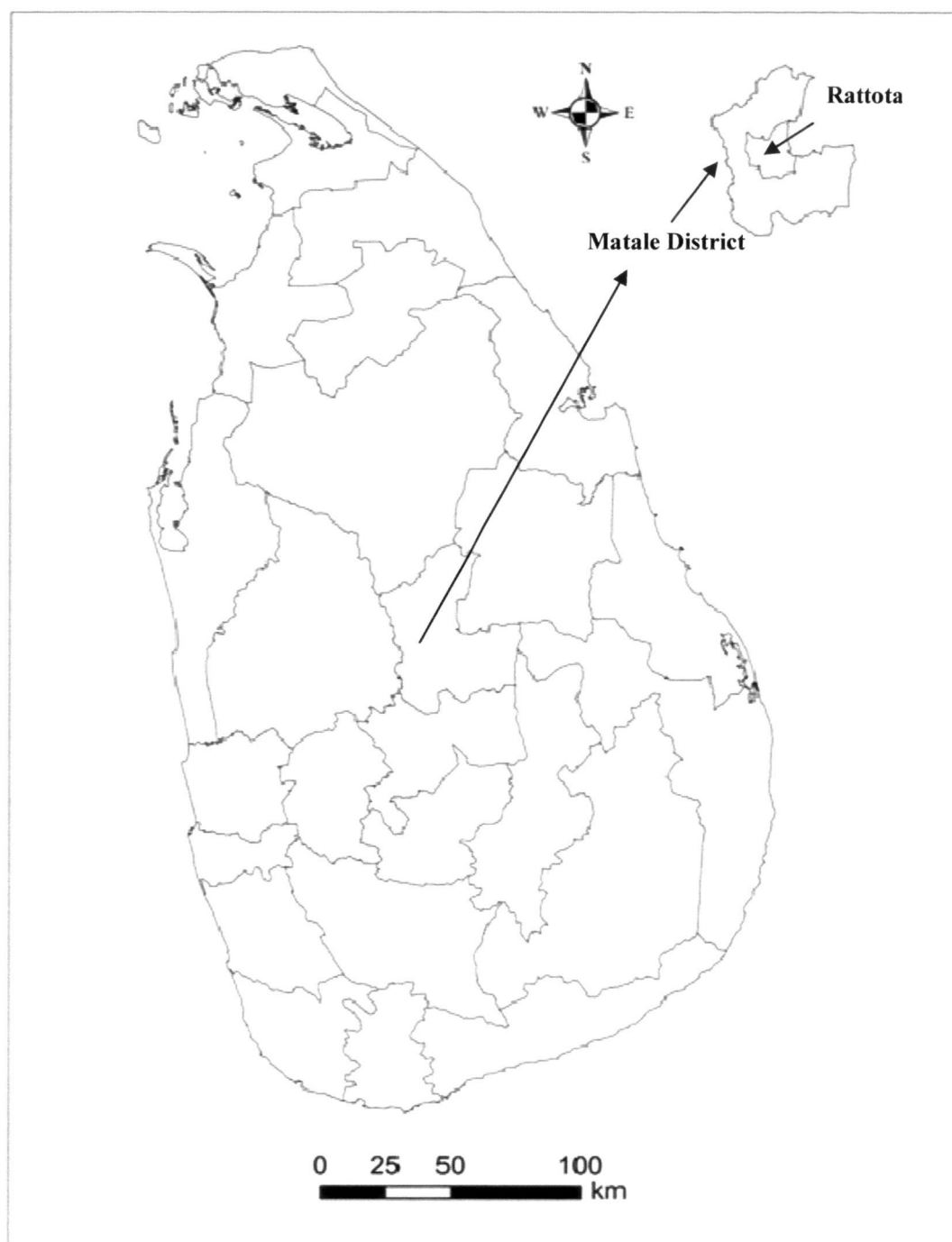
Figure 2: Location of the Nikola Oya landslide at Rattota Divisional Secretariat Area
