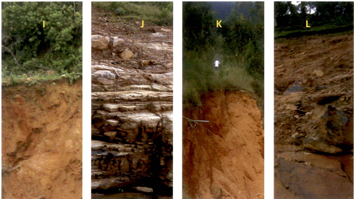
Figure 7: Photos I – L shows the unstable conditions of soil strata along the Nikola Oya basin.
